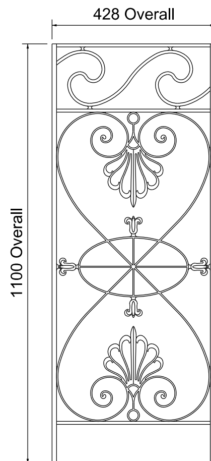
ELEVATION OF SMALL 'CHELTENHAM' CAST BALUSTRADE PANEL
