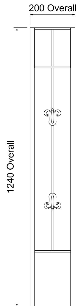
ELEVATION OF 'CHELTENHAM' CAST BALUSTRADE POST
