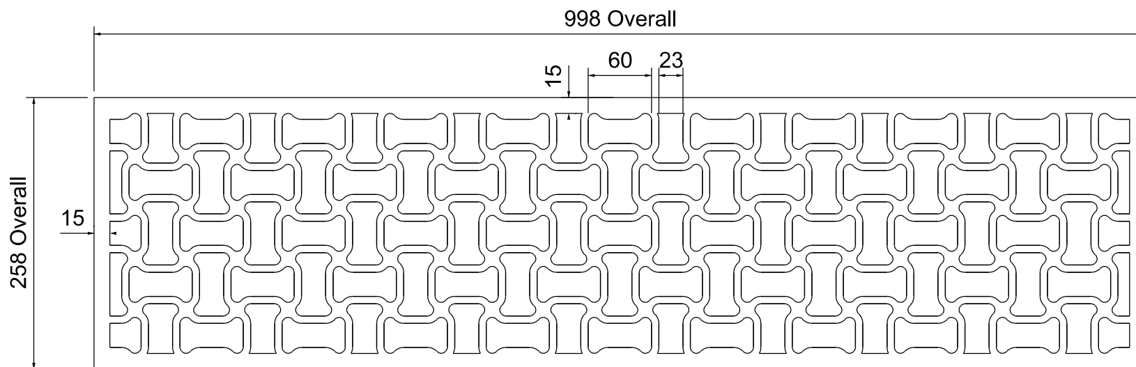
ELEVATION OF GRILLE
