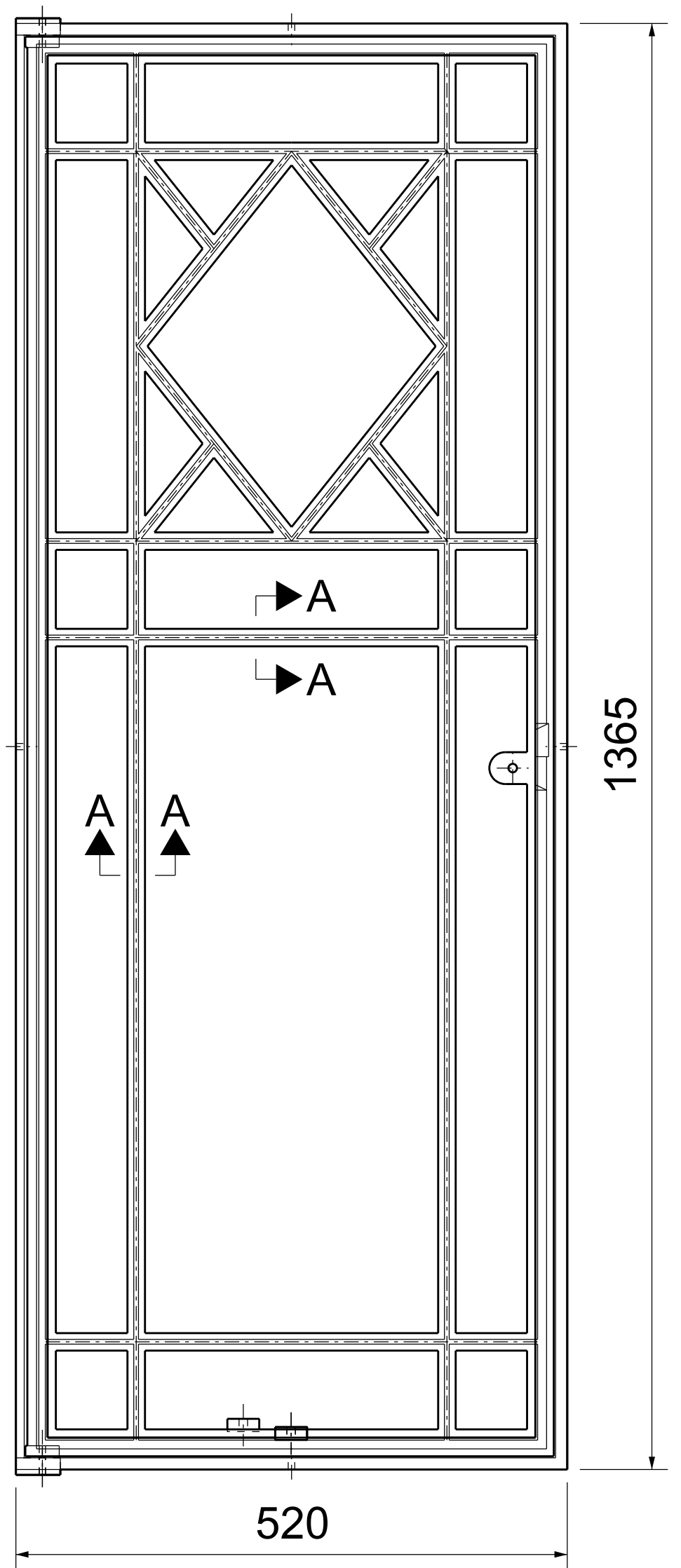
CAST OPENING WINDOW SCALE 1:5 @ A3
